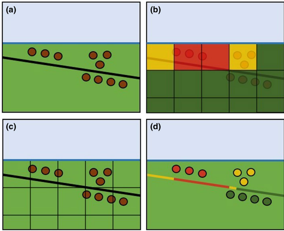
Fig. 1 A hypothetical coastal example of how the CESM score is assigned to asset data, a a rail track (black line), and dwellings (brown circles) are located at the coast, b the 50 m 2 CESM raster for the same area shows areas of very high susceptibility (red grid cells), high susceptibility (yellow grid cells), and very low susceptibility (green grid cells), c the raster is converted to a polygon, then intersected with the asset data which has the effect of assigning the values of the 50 m 2 raster grid to the asset data, d the CESM values have been assigned to the asset data with lengths of the rail track and dwellings classified as exposed (red lengths of rail track and red dwellings)
