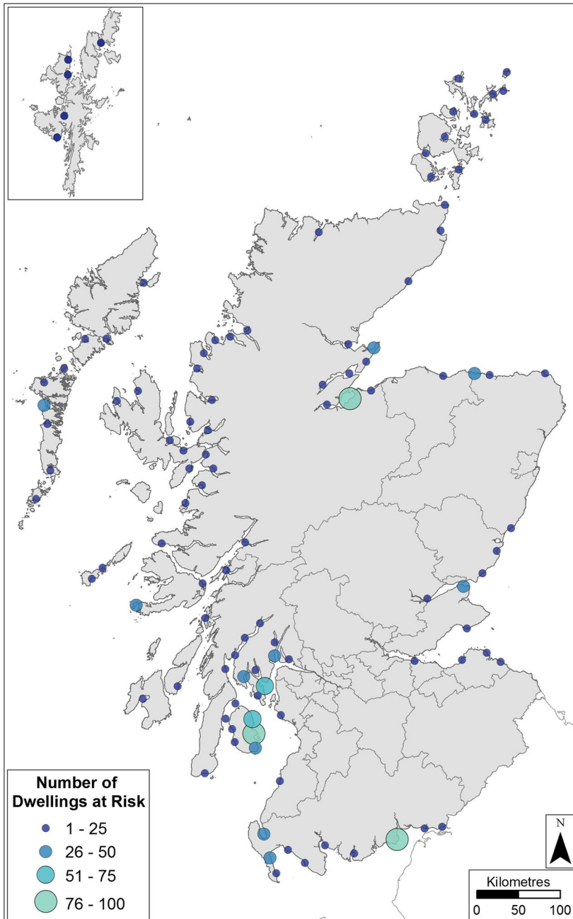
Fig. 4 The location of the 1273 high-risk dwellings which are classified as exposed ( \text{CESM} \geq 80 ) and have very high vulnerability according to the CEVI [Very High (red) areas in Fig. 3]. In contrast to Fig. 3, where the entirety of Scotland was classified with a degree of vulnerability, the addition of the CESM has confined the risk to dwellings at the coast
