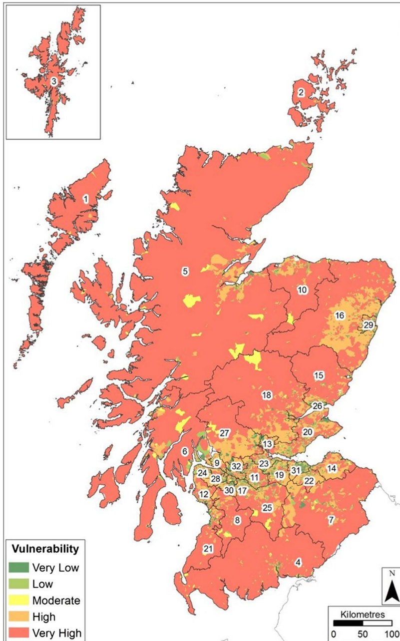
Fig. 3 The Coastal Erosion Vulnerability Index (CEVI) for Scotland. Although the CEVI has been tailored for coastal erosion, areas of the hinterland that are some distance from the coast are classified with very high vulnerability, which may appear counter-intuitive. However, as stated in Sect. 1.1, vulnerability is defined as being independent of the geographical extent of the coastal erosion hazard; therefore, it is only when the CESM is used along with the CEVI (as shown in Fig. 4) is risk confined to the coast. Numbering refers to the local authorities in Table 11. This map is viewable in greater detail via a webmap at www.jmfiton.xyz/cer
